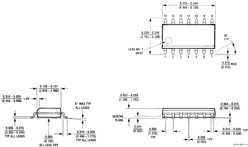
14-Lead Small Outline Molded Package (M) Order Number DM74LS74AM NS Package Number M14A
